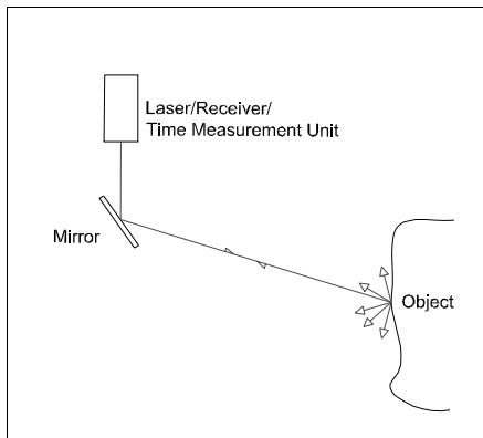
Figure 1: Time-of-flight
