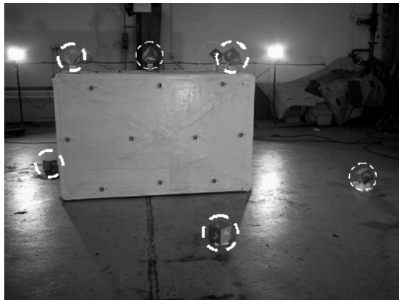
Fig. 8: images with perpendicular viewing directions and detected tie objects
