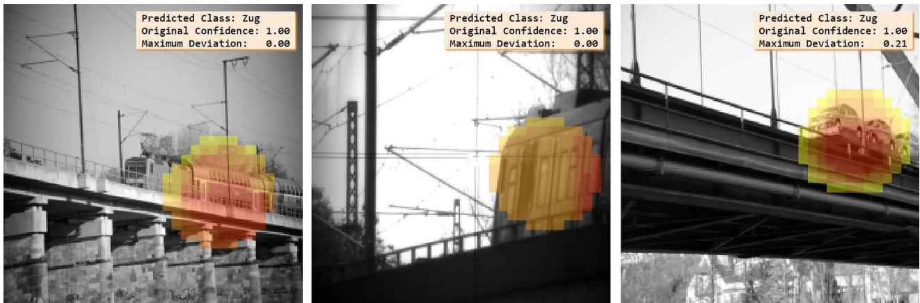
Abb. 5: MVTec Heatmaps
