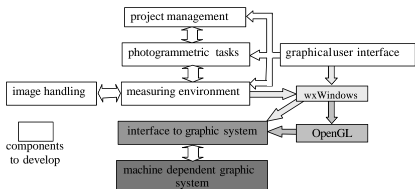
Figure 2: structure of software
