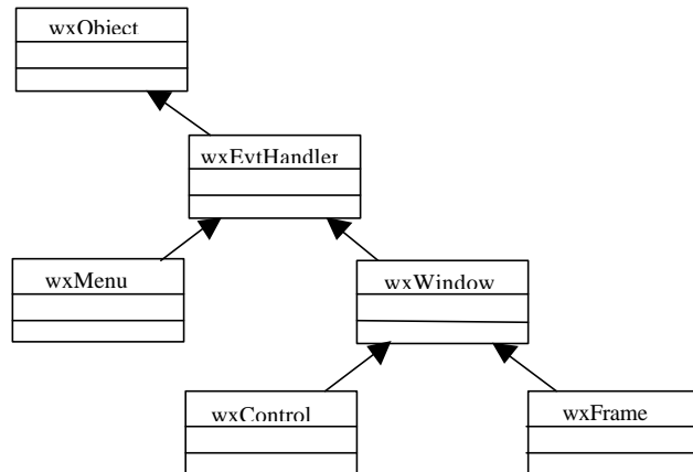
Figure 3: Simple UML showing some wxWindows classes
