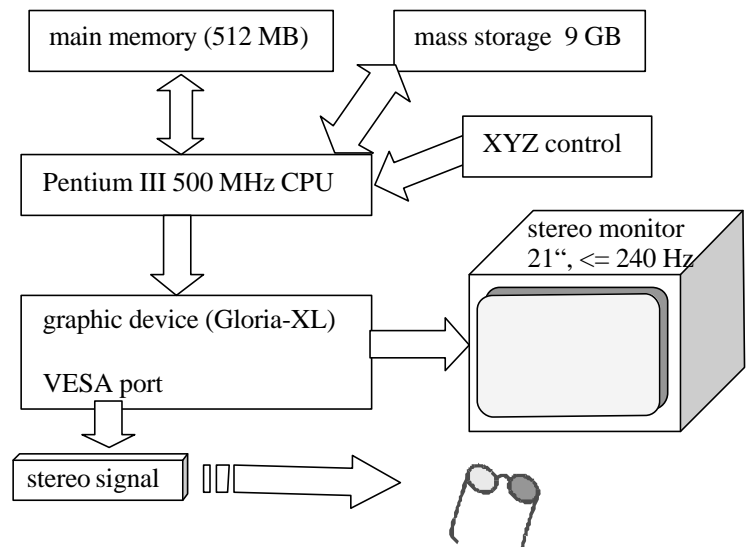
Figure 1: system components
