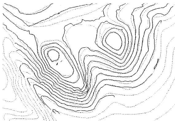
Figure 6. Overlay of contour lines generated from 1/5000 scale TIN (dashed lines) and from 1/500 scale TIN (solid lines).
